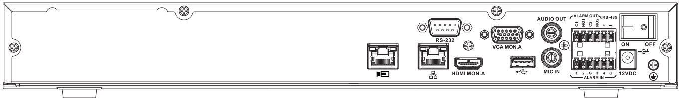
Fig. 1: DIVAR network 2000 (no PoE) back panel
