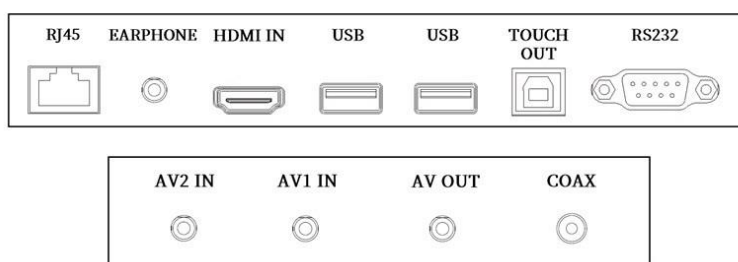
Side Interfaces:
